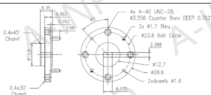
FUGP500 (equivalent to UG-383/U-M)
