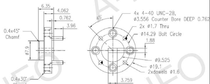
FUGP620 (equivalent to UG-385/U)
