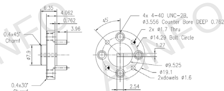
FUGP900 (equivalent to UG-387/U-M)
